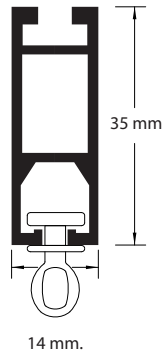
W = 14 mm. H = 35 mm. Thickness 1.2 Aluminium track
